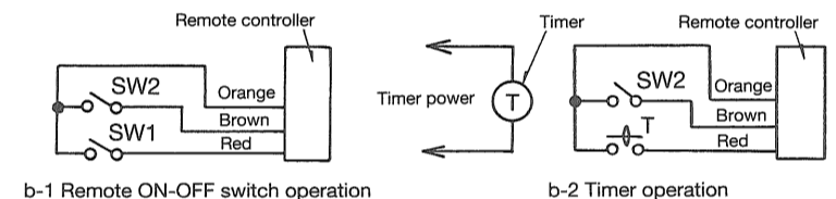
b-1 Remote ON-OFF switch operation
