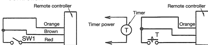
a-1 Remote ON-OFF switch operation
